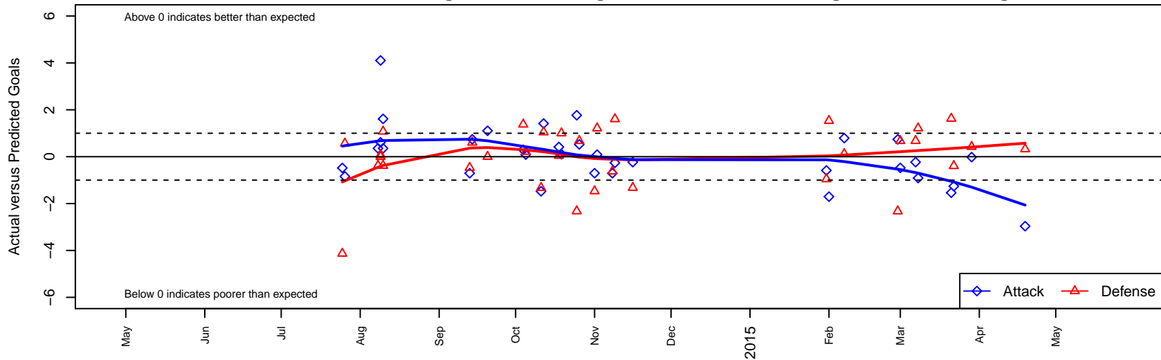
SSC Shadow B B01 Dots are actual minus expected GF (blue circles) and GA (red triangles). Blue line is smoothed change in attack strength. Red is smoothed change in defense strength.
